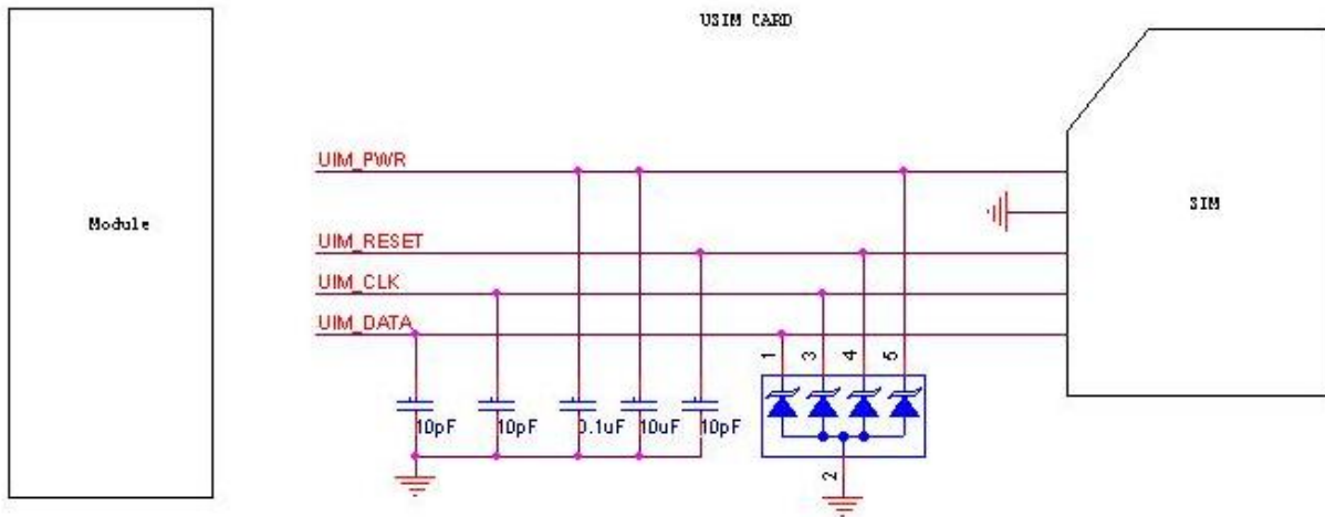
Figure 4-1 USIM card interface circuit schematic diagram
